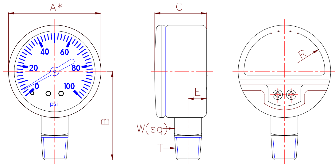
Lower Mount (LM)
